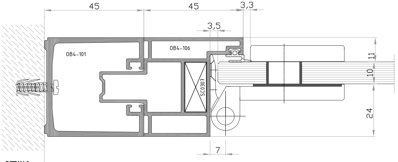
DETAY-2
