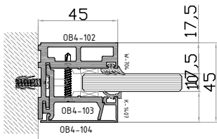
1-DETAY
