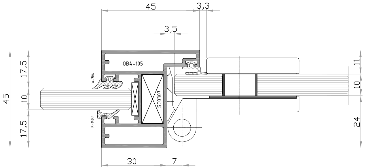
DETAY-1
